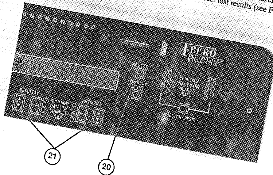
Figure 4-8 Controls to Start Tests and Collect Results
