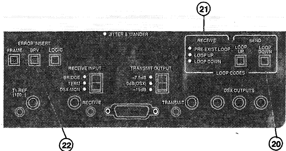
Figure 3-7 Troubleshooting Controls
