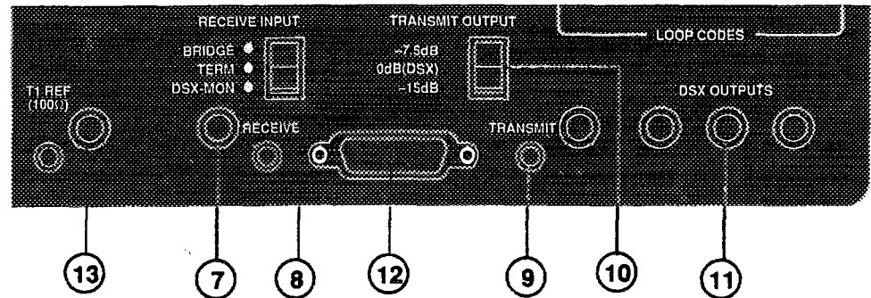
Figure 3-4 Front-Panel Connections
