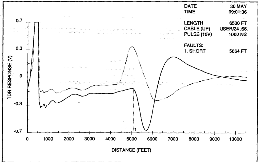
Figure 7-8 Dual Trace TDR GRAPH
