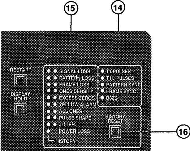
Figure 3-5 Signal Verification Indicators
