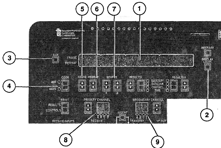
Figure 4-5 Test Setup Controls and Indicators
