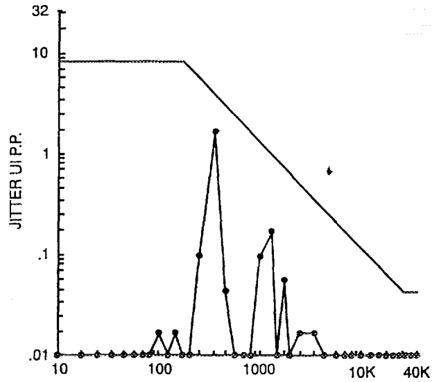
Figure 3-9 Sample Jitter vs Frequency Graph
