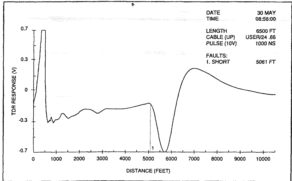
Figure 7-7 Single Trace TDR GRAPH
